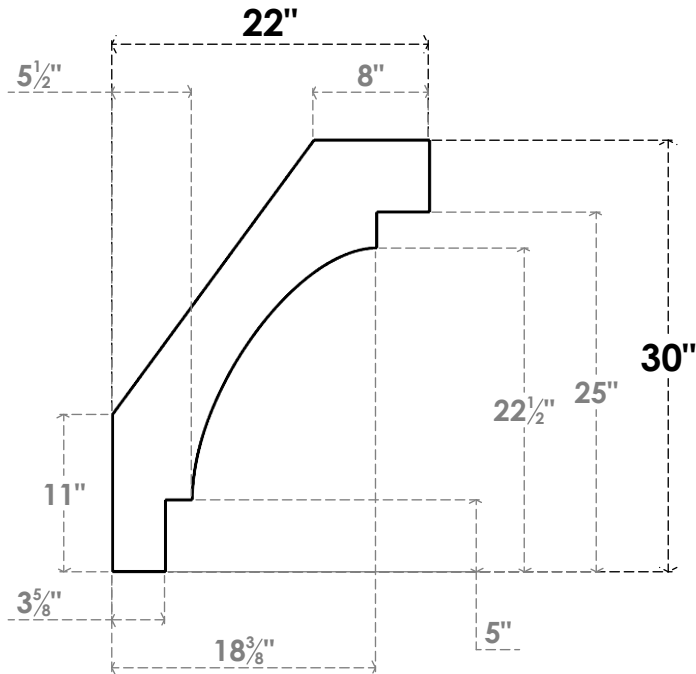
SIDE PROFILE
